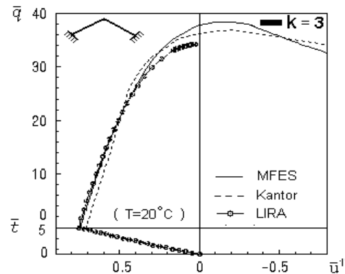
Figure 2 – The “ \bar{q} - \bar{u}' ” curves for preheated conical panel
